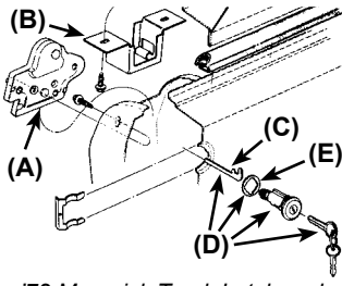
'72 Maverick Trunk Latch and Lock Assembly
