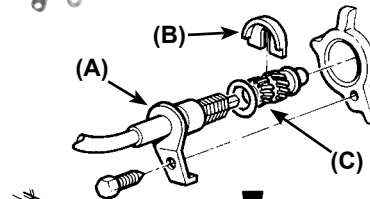
Typical Lower Speedometer Cable Assembly
