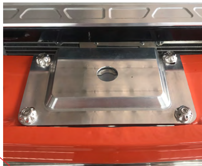
Hood latch billet Chevy C10
